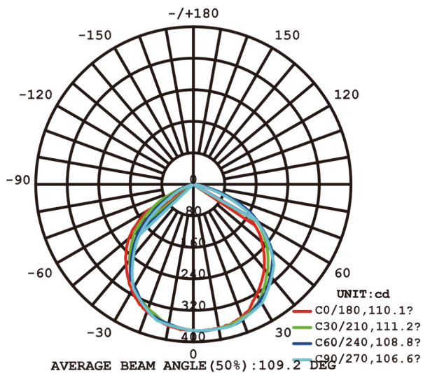
PHOTOMETRIC DIAGRAM
