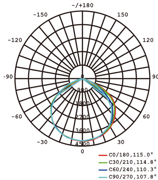
PHOTOMETRIC DIAGRAM
