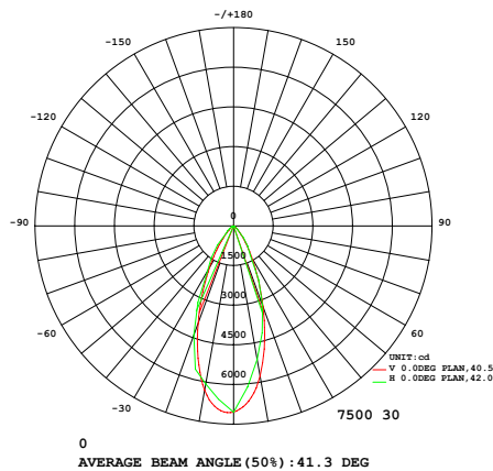
PHOTOMETRIC DIAGRAM
