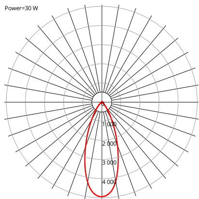
PHOTOMETRIC DIAGRAM
