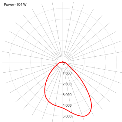
PHOTOMETRIC DIAGRAM
